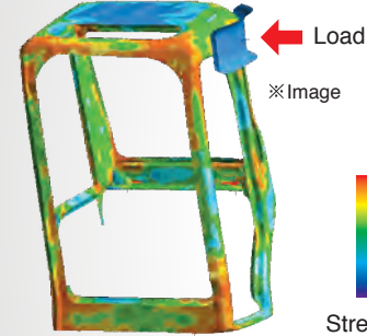
FOPS-1 stress analysis graph
