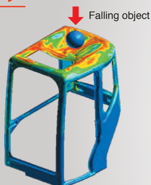
ROPS stress analysis graph
